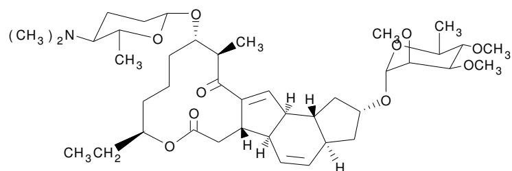
spinosyn A
