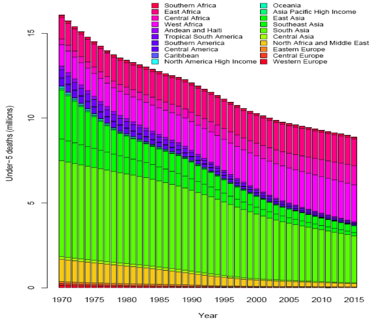
Figure 4: Regional composition of the estimated global time-trend in under-5 deaths.
