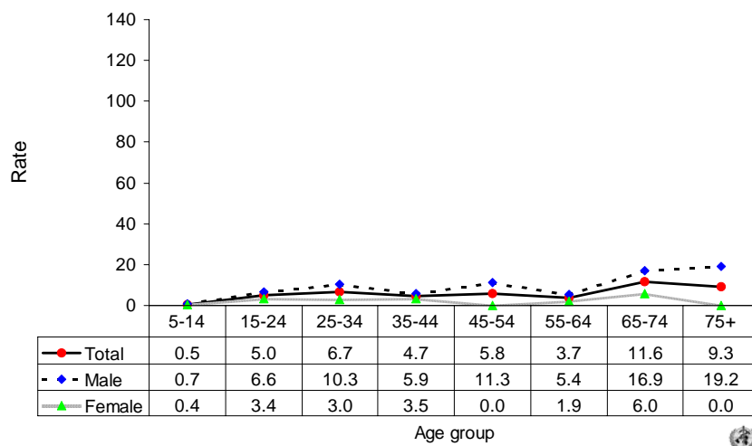
Suicide rates (per 100,000), by gender and age, Panama, 1987.
