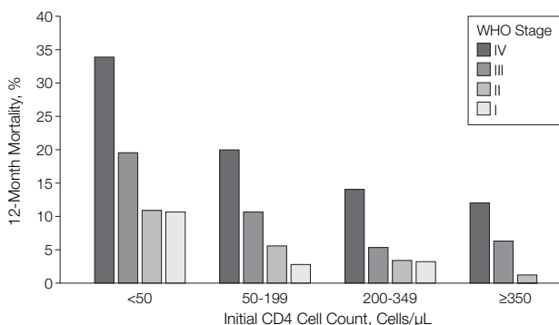
Figure 4. One-Year Mortality Among Patients Starting Antiretroviral Therapy by Initial CD4 Cell Count and WHO Stage, Lusaka, Zambia (April 2004–November 2005)
