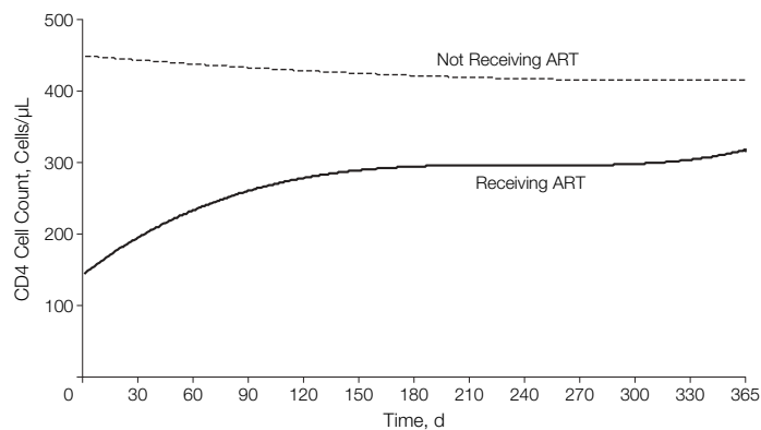
Figure 5. Modeled Changes in CD4 Cell Count Over Time for Surviving Patients Who Received or Did Not Receive Antiretroviral Therapy, Lusaka, Zambia (April 2004–November 2005)
