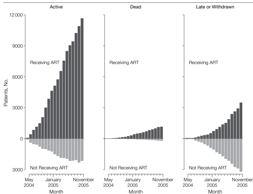
Figure 2. Cumulative Status Over Time of Participants in the Antiretroviral Therapy Program, Lusaka, Zambia (April 2004–November 2005)
