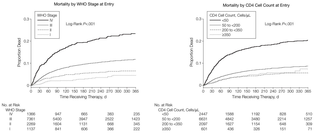
Figure 3. One-Year Mortality of Patients Starting Antiretroviral Therapy by Initial WHO Clinical Stage and CD4 Cell Count, Lusaka, Zambia (April 2004-November 2005)
