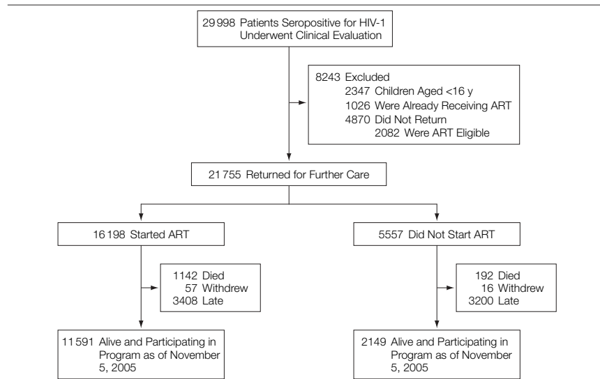
Figure 1. Description of an Antiretroviral Therapy Program Cohort, Lusaka, Zambia (April 2004–November 2005)
